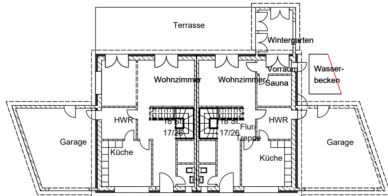
Erdgeschoss M=1:200
